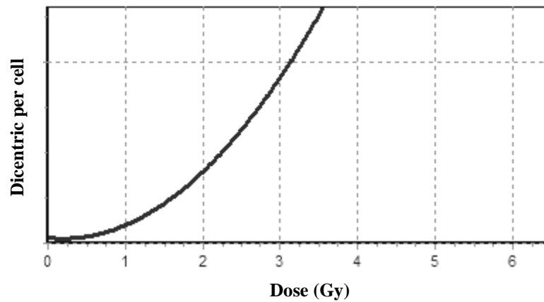
Figure 1 - Dose-response curve generated by CABAS
